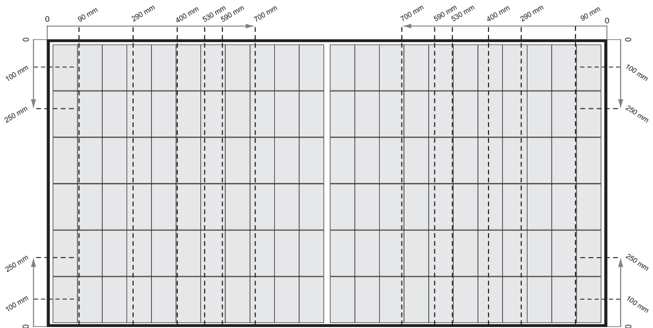
Fig. 3-1 Clamping of REC Alpha Pure 2 Series panels with Rails parallel to the Short Side of the Panel
