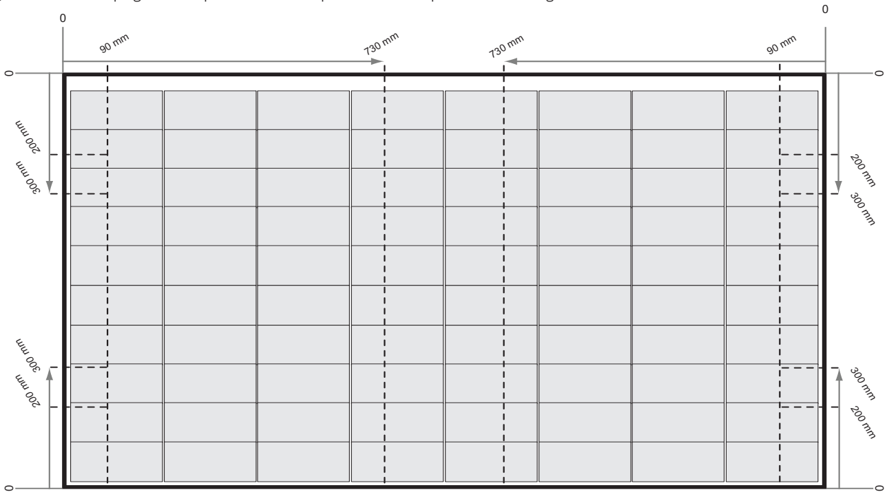
Fig. 4-2 Clamping of REC Alpha Pure-R Series panels with Rails parallel to the Long Side of the Panel
