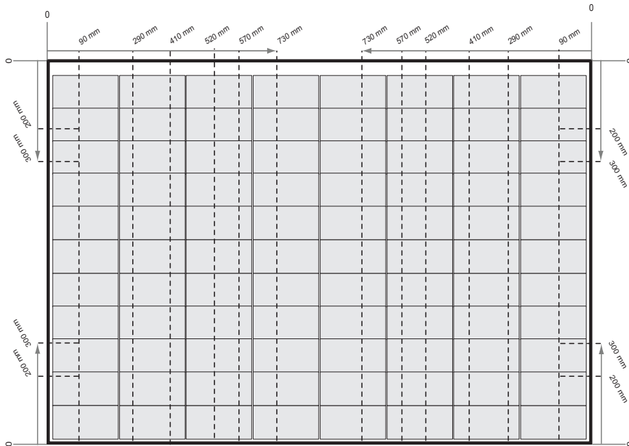
Fig. 5-1 Clamping of REC Alpha Pure-RX Series panels with Rails parallel to the Short Side of the Panel
