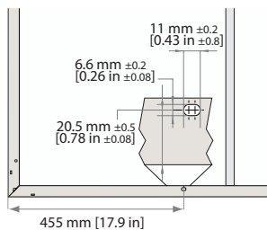
Fig. 3 Mounting holes: REC Alpha Panels
