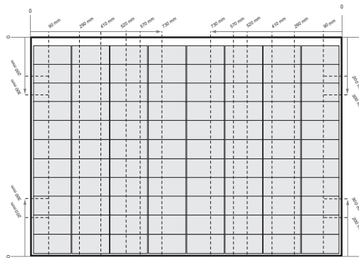
Fig. 5-3 Clamping of REC Alpha Pure-RX Series panels using short rails
