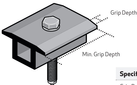
Fig. 1 Clamp Specifications
