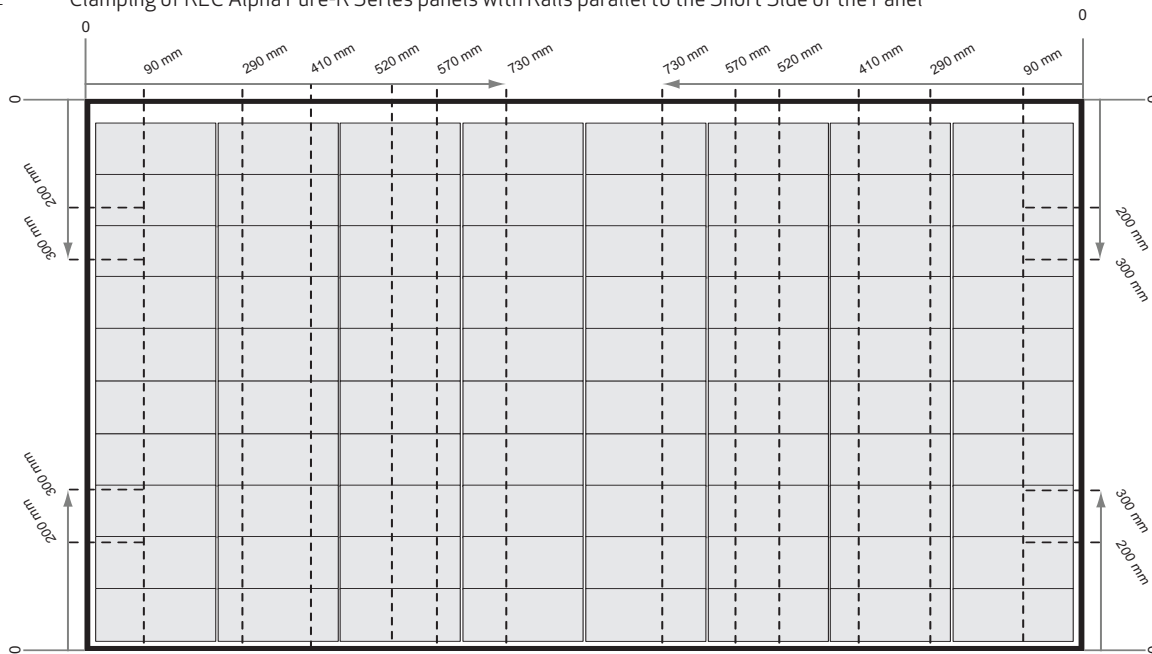
Fig. 4-1 Clamping of REC Alpha Pure-R Series panels with Rails parallel to the Short Side of the Panel
