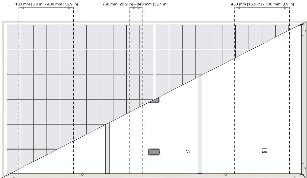
Fig. 2-4 Six-point mounting configuration clamping zones: REC Alpha Pure Series
