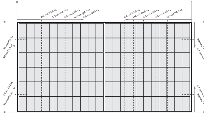
Fig. 2-3 Clamping of REC Alpha Pure Series panels using short rails
