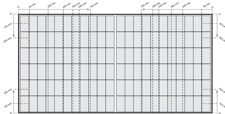
Fig. 3-3 Clamping of REC Alpha Pure 2 Series panels using short rails
