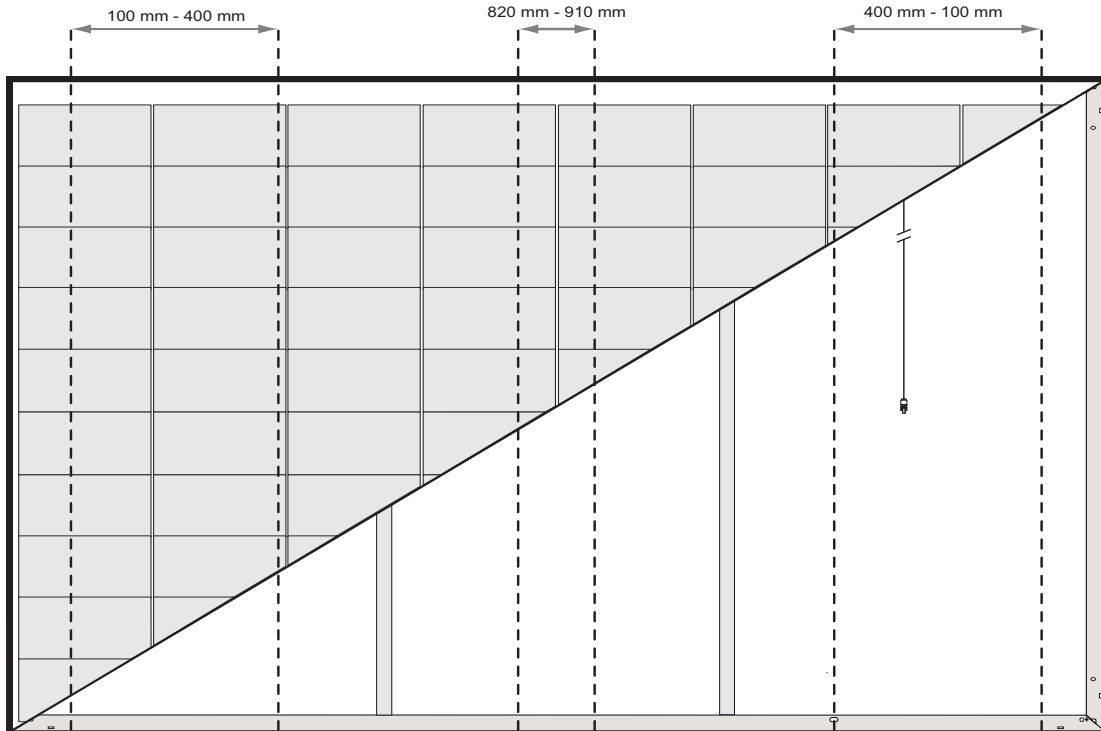
Fig. 4-4 Six-point mounting configuration clamping zones: REC Alpha Pure-R Series
