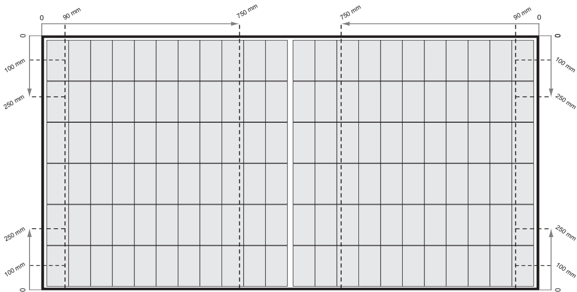
Fig. 3-2 Clamping of REC Alpha Pure 2 Series panels with Rails parallel to the Long Side of the Panel
