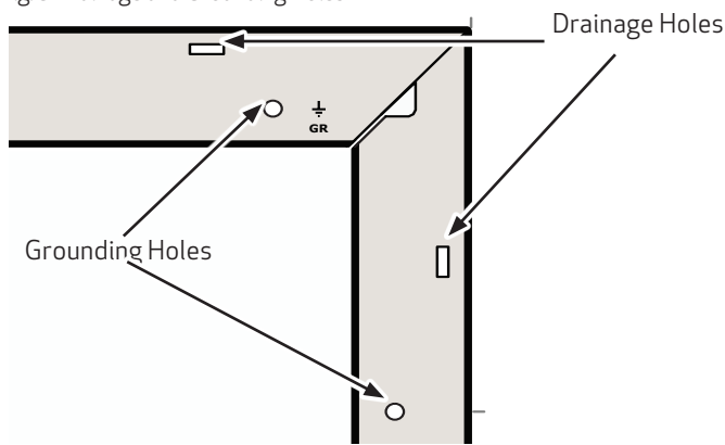
Fig. 5 Drainage and Grounding Holes
