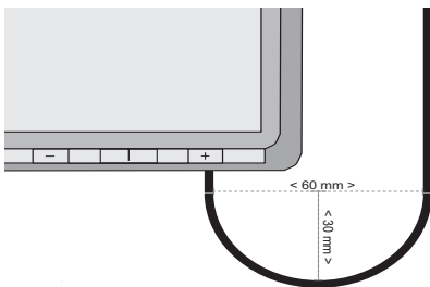
Fig. 6 Minimum Cable Distance
