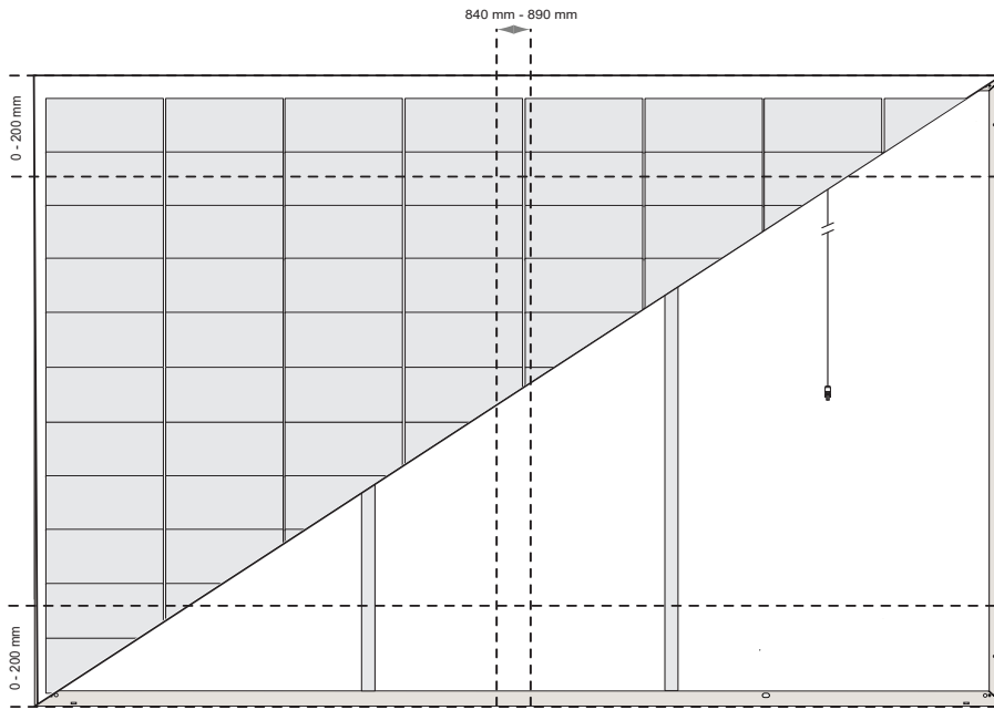
Fig. 5-5 Mixed Six-Point Mounting of REC Alpha Pure-RX Series Panels using short rails
