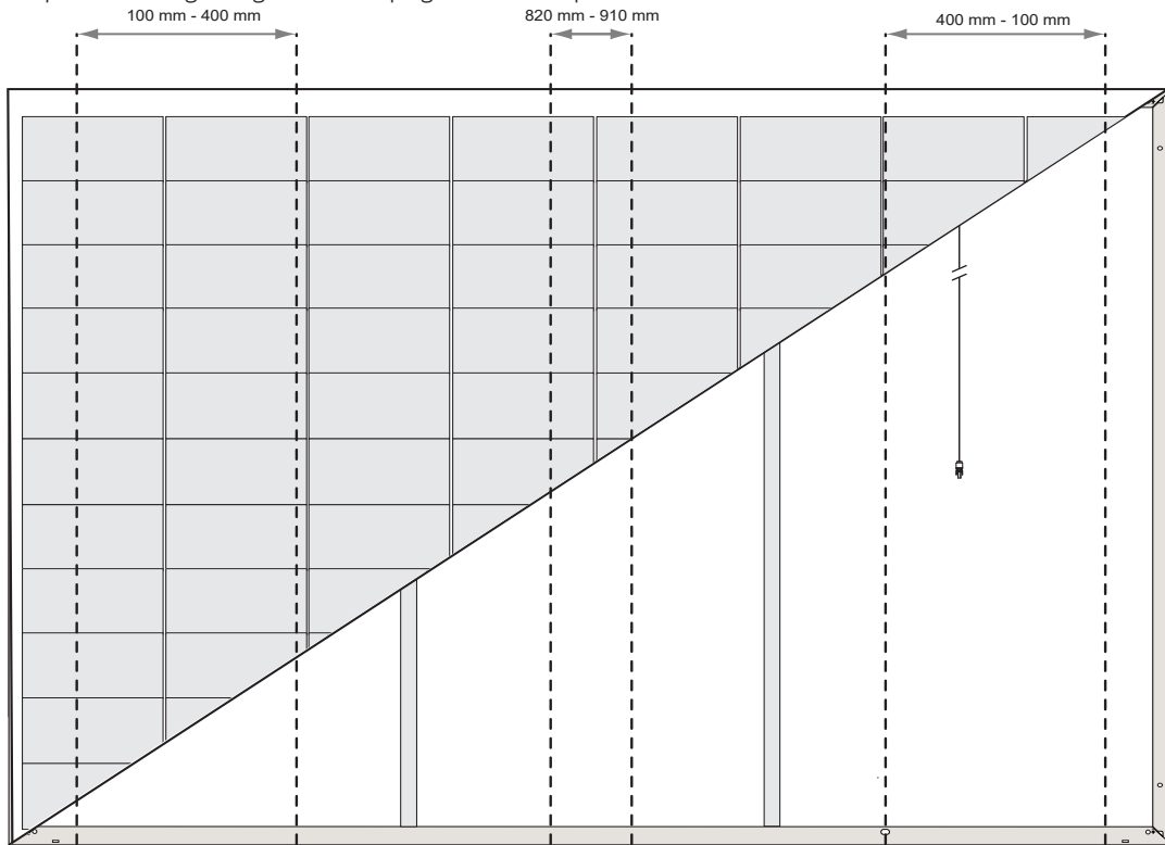
Fig. 5-4 Six-point mounting configuration clamping zones: REC Alpha Pure-RX Series
