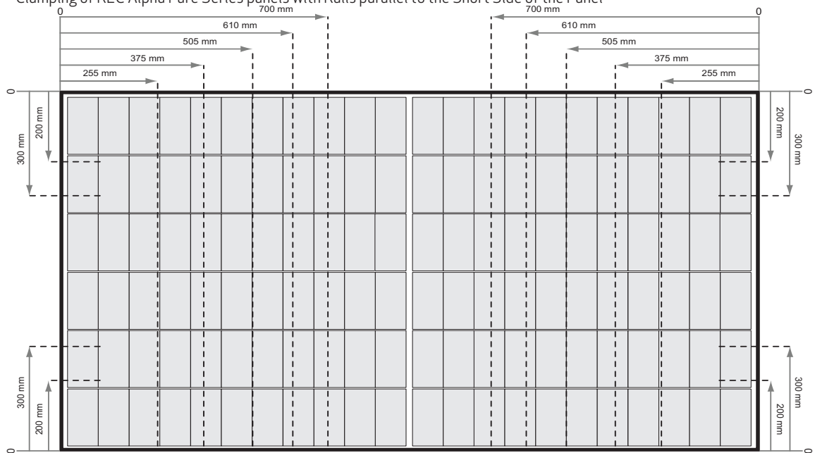
Fig. 2-1 Clamping of REC Alpha Pure Series panels with Rails parallel to the Short Side of the Panel
