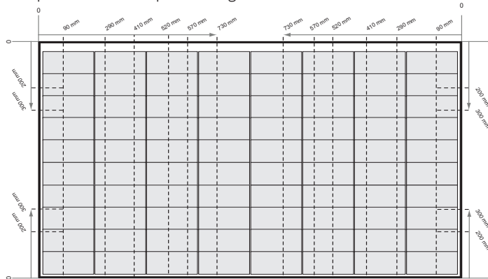
Fig. 4-3 Clamping of REC Alpha Pure-R Series panels using short rails
