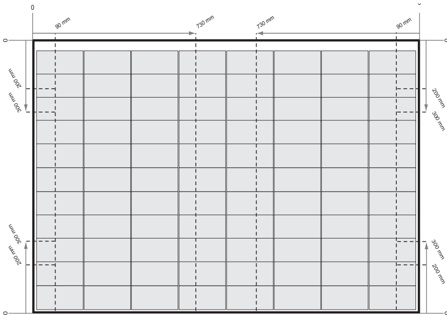
Fig. 5-2 Clamping of REC Alpha Pure-RX Series panels with Rails parallel to the Long Side of the Panel
