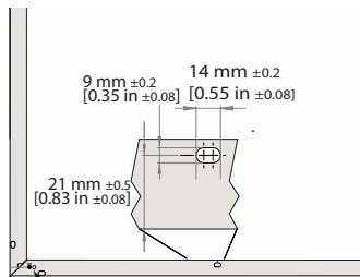
Fig. 3 Mounting holes: REC Alpha Panels
