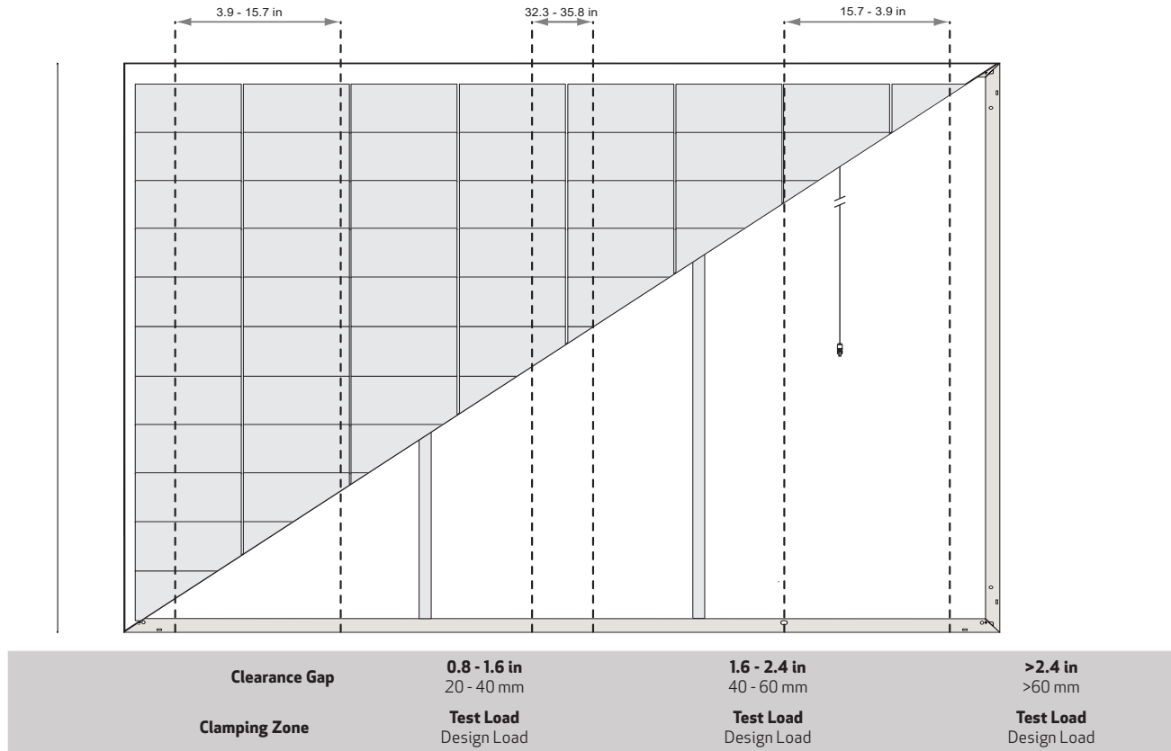
Fig. 5-4 Six-point mounting configuration clamping zones: REC Alpha Pure-RX Series
