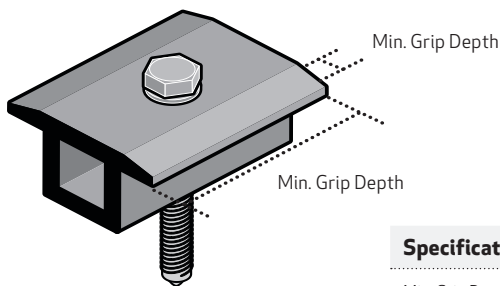
Fig. 1 Clamp Specifications
