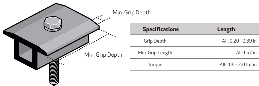
Fig. 1 Clamp Specifications
